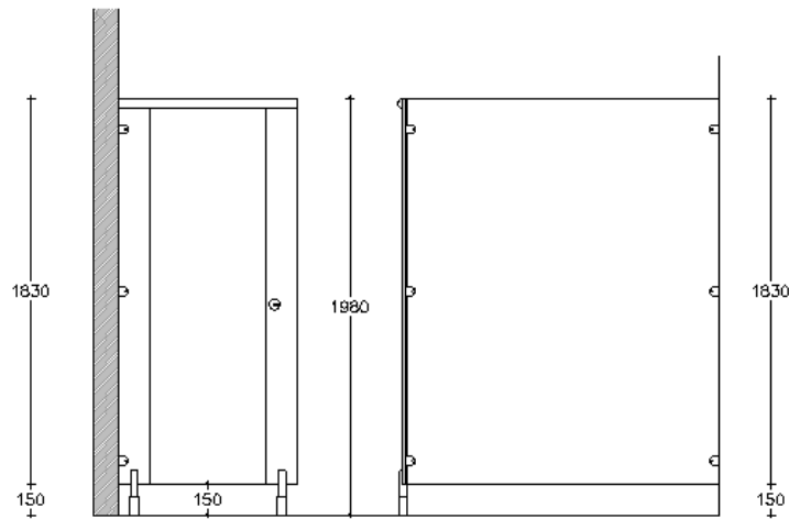
Typical Cubicle Elevations
